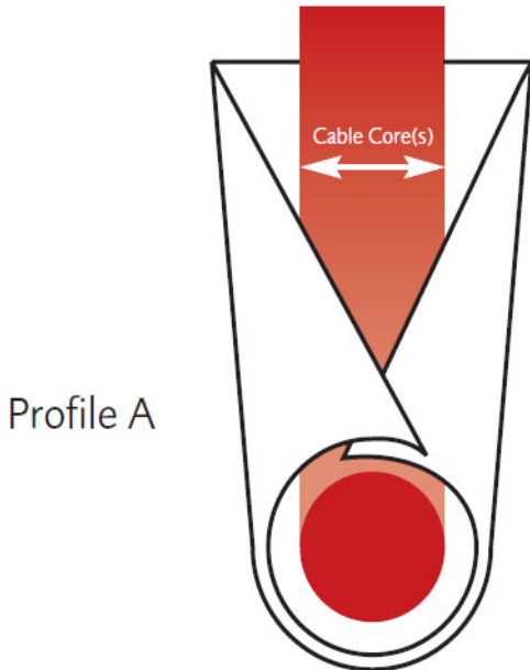
Exit of tape former cable, with tape security wrapped around it.
